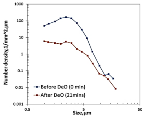
Figure 1 Size distribution of FeO inclusions before and Al 2 O 3 inclusions after deoxidation (Figure shows similarities in both shape and size range)
