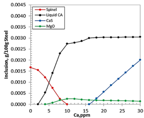
Figure 6 Thermodynamic calculation showing the formation of MgO during calcium modification of MgO saturated spinel
