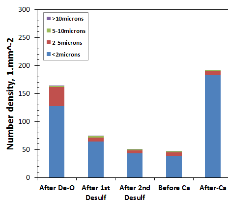
Figure 3 Reduction in number density with time due to argon stirring in a mini mill
