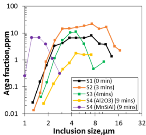
Figure 7 Change in inclusion composition and size distribution resulting from steel reoxidation
