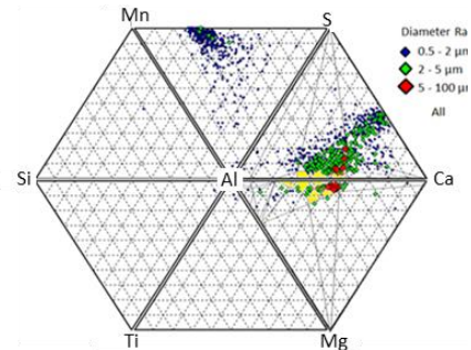
Figure 8 Inclusion composition during ladle transfer (Modified calcium aluminates are observed and result from CaS reaction with newly formed inclusions after reoxidation)
