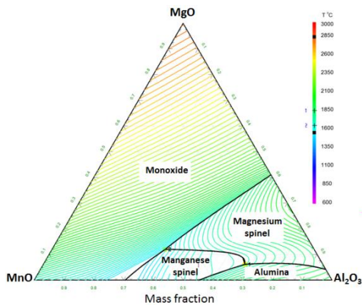
Figure 5 Phase diagram of the MnO-MgO-Al 2 O 3 system
