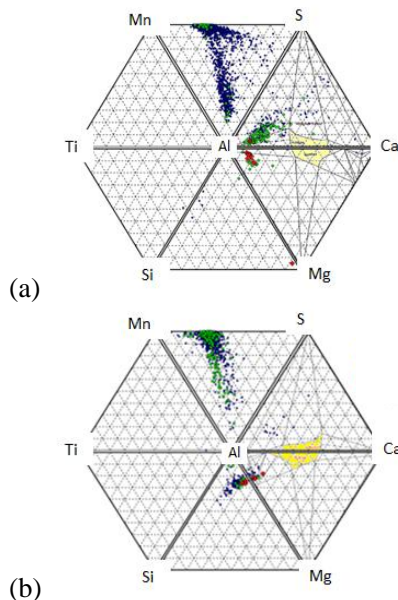
Figure 2. Inclusion composition observed after deoxidation in (a) plant ‘A’, and (b) plant ‘B’ (Plant A contained mainly calcium aluminate and plant B contained magnesium spinels)
