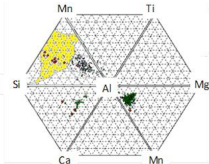
Figure 4 Inclusion composition showing presence of manganese aluminates at a BOP facility
