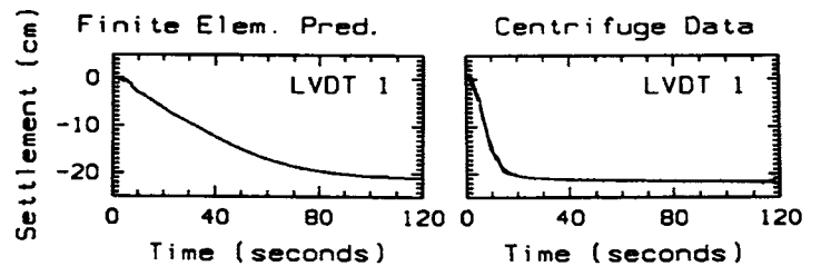
Fig. 7. Ground Settlement History.
