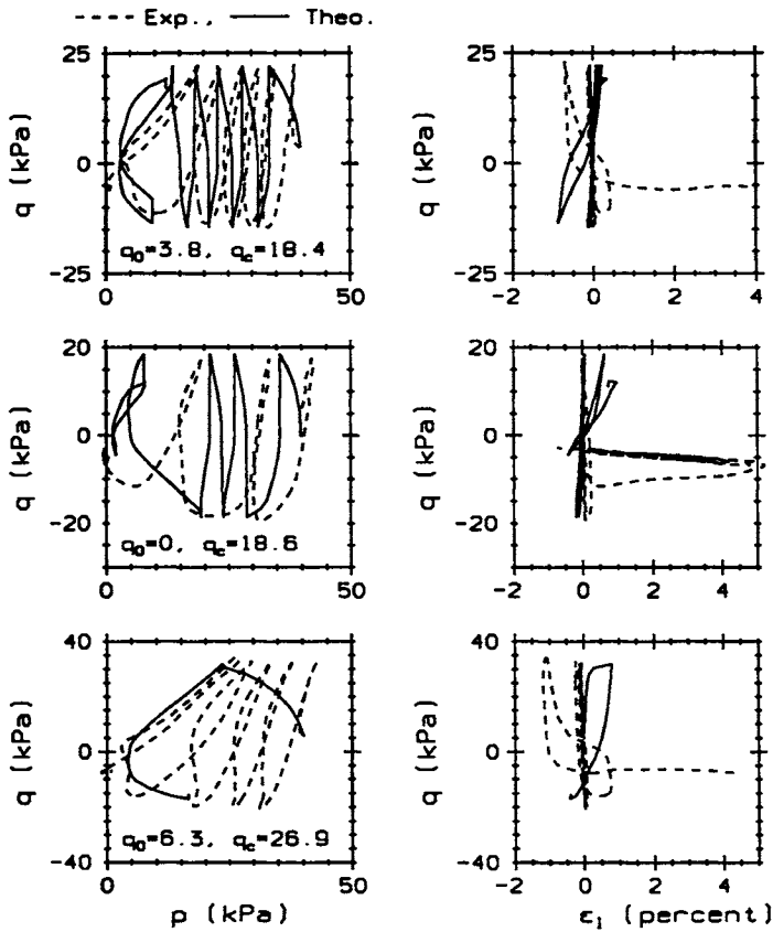
Fig. 1. Comparison of the Model Behavior with Experimental Data of Cyclic Triaxial Behavior of Nevada Sand of Dr=40 percent at p₀=40 kPa.
