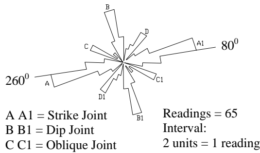
Fig.6. Rose diagram of joints in porphyritic granite at Kalapahar Landslide
