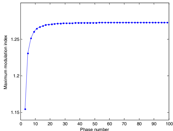
Figure 3. Maximum modulation index verse phase number.
