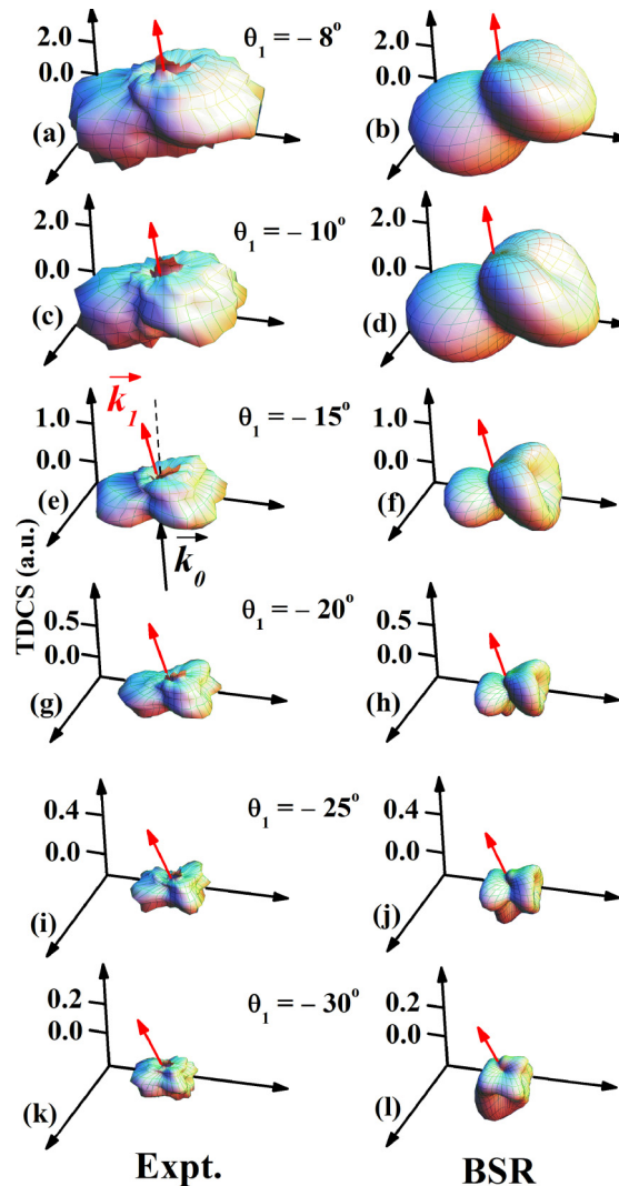
FIG. 2. (Color online) Three-dimensional presentation of the triple-differential cross section for single ionization of Ar ( 3p ) by 70.8 eV electron impact as a function of the emission angle of an electron with kinetic energy E_2 = 3 eV ( \pm 1.0 eV) and different projectile scattering angles ( \theta_1 ). (a) and (b) \theta_1 = -8^\circ ( \pm 1.5^\circ ), (c) and (d) \theta_1 = -10^\circ ( \pm 2.0^\circ ), (e) and (f) \theta_1 = -15^\circ ( \pm 2.5^\circ ), (g) and (h) \theta_1 = -20^\circ ( \pm 3.0^\circ ), (i) and (j) \theta_1 = -25^\circ ( \pm 3.0^\circ ), and (k) and (l) \theta_1 = -30^\circ ( \pm 3.5^\circ ). Left column: experiment. Right column: B -spline R -matrix with pseudostates (BSR) theory.
