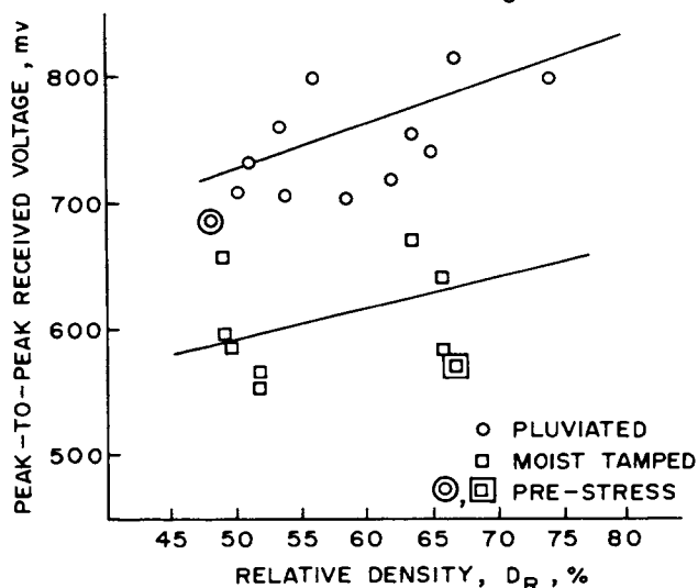
Figure 3. Signal Attenuation Versus Relative Density, Dover 40-50 Sand
