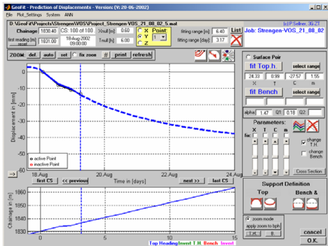
Fig. 6. Prediction of displacements at the Strenger tunnel; the dashed line indicates the predicted development of the displacements
