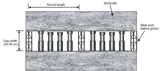
Fig 11. Typical assembly of LSC groups between steel arches
