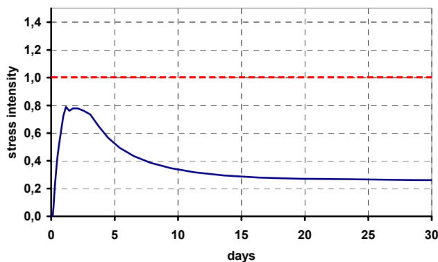
Fig. 14. Development of the stress intensity factor for the same rock mass conditions, but with higher advance rate
