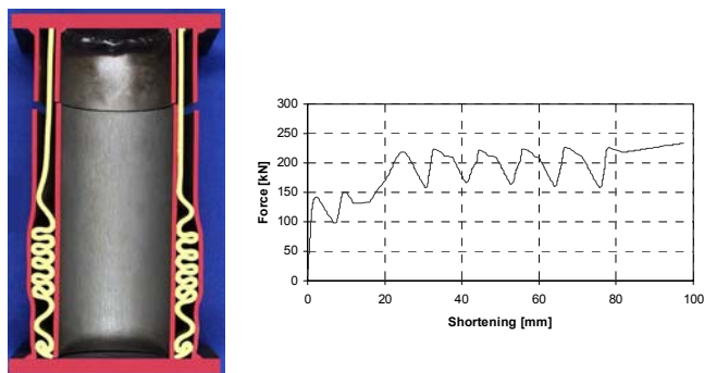
Fig. 10. Yielding element after laboratory testing (left), and load line (right)
