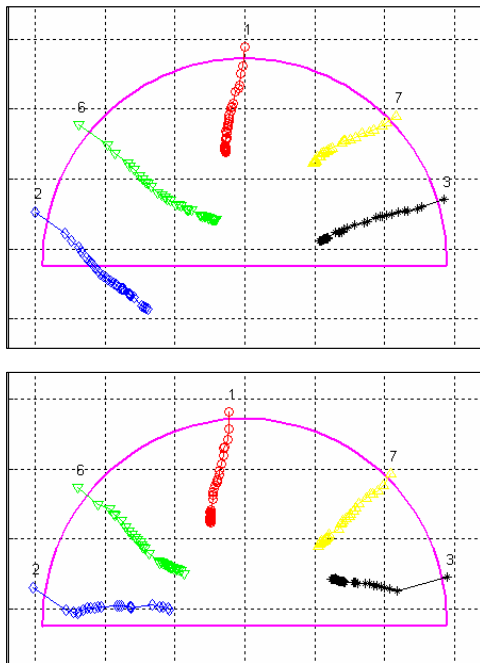
Fig. 2. Displacement vector plots of two measuring sections with a distance of 10 m, showing different behaviour
