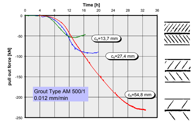
Fig. 9. Performance characteristic of 3 bolts with different rib distance, using the same grout type and displacement rate
