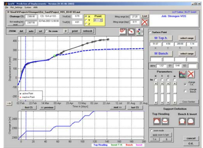
Fig. 8. Deviation of the measured horizontal displacements of left sidewall point from the predicted ones due to failure of the invert (Strenger tunnel, Austria).
