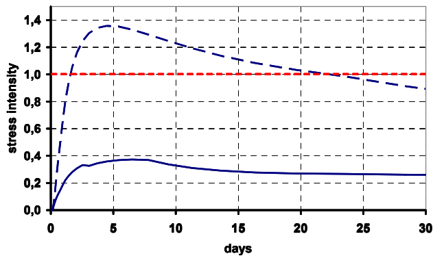
Fig. 13. Development of stress intensity factor in the shotcrete lining without (dashed line) and with yielding elements (solid line)
