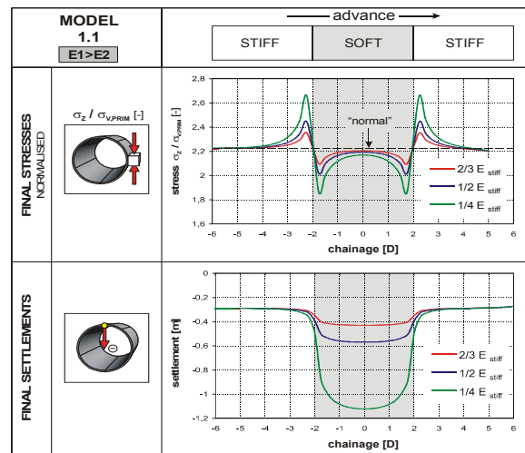
Fig. 3. Arching effect in a weak zone leading to stress concentrations in the stiffer material at the boundaries and the typical trough shaped displacement distribution (numerical model).
