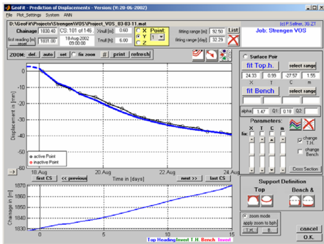
Fig. 7. Comparison between predicted and measured values at the Strenger tunnel.
