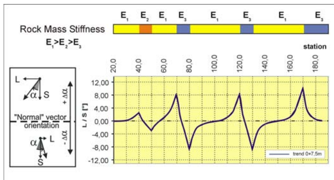
Fig. 4. Variation of displacement vector orientation when tunnelling in a heterogeneous rock mass, result of numerical simulation
