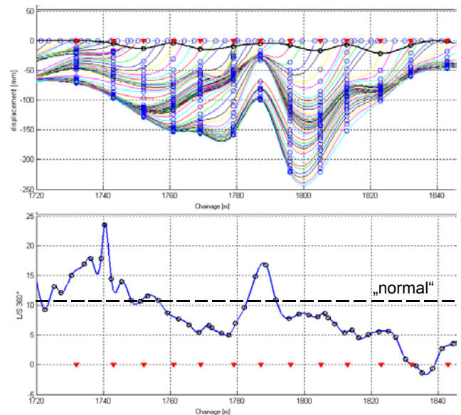
Fig. 5. Settlements and displacement vector orientation trend for a side wall point at the tunnel Spital, Austria.
