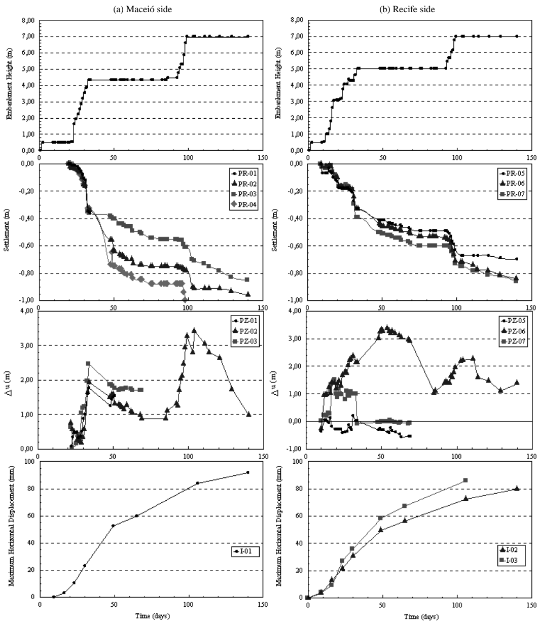
Figure 2 - Results of the geotechnical instrumentation measurements - embankments of access of the Bridge on Jituba River.
