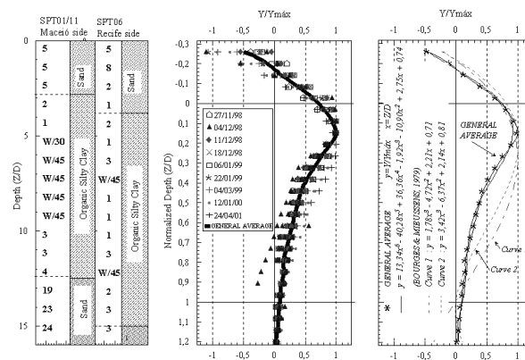
Figure 8 - Comparison of the average of the profiles normalized with the curves proposed by BOURGES & MIEUSSENS (1979).
