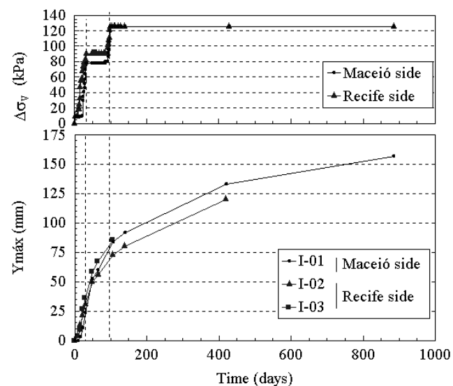
Figure 9 - Maximum horizontal displacements with time - up to period 885 days.
