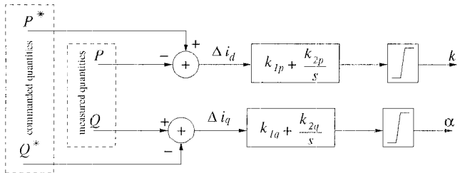
Figure 2 – PQ Decoupled PI Control Block Diagram for StatCom/BESS
