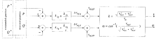
Figure 3 – PQ Decoupled PI Control Block Diagram for SSSC/BESS
