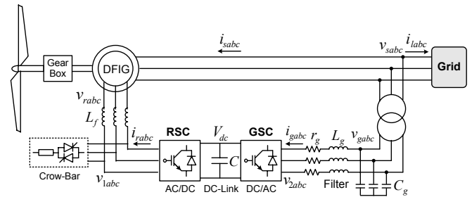
Fig. 2. Aggregated wind farm model: one equivalent DFIG driven by a single equivalent wind turbine.
