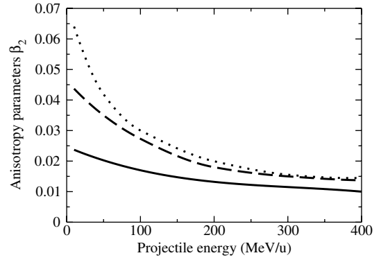
FIG. 4. Anisotropy parameters of the K\alpha_1 radiation following REC into the 1s_{1/2}2p_{3/2}^1,3P_{J=1,2} levels of the (finally) heliumlike xenon Xe^{52+} (dotted line), gold Au^{77+} (dashed line), and uranium U^{90+} (solid line) ions. All results include the feeding transitions from the higher excited states.
