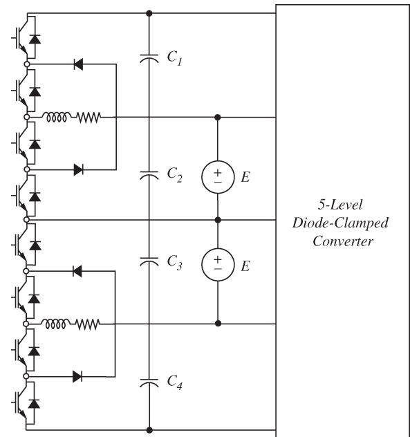
Fig. 5. Balancing circuit for five-level diode-clamped STATCOM/2 BESS converter.
