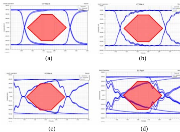
Fig. 11 Simulated eye-diagram : (a) without varistor; (b) with 4 pF varistor; (c) with 20 pF varistor; (d) with 40 pF varistor
