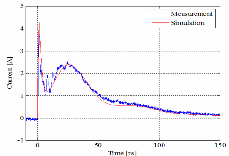
Fig. 8 ESD current waveform comparison
