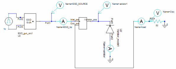
Fig. 6 Full circuit model of a PCB with the ESD generator and varistor
