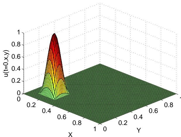
Figure 4: Surface plot of initial condition (38) used in the GFE simulation of Burgers' equation
