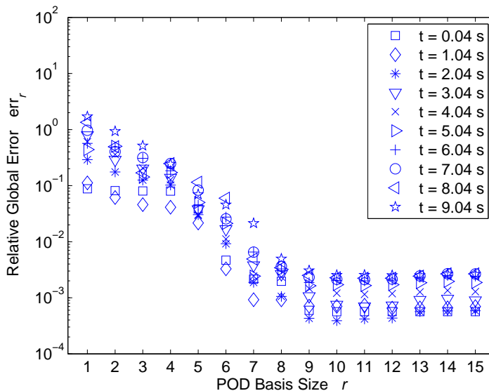
Figure 2: Semilog plot of relative global error versus POD basis size at various points in time for the simulation of the group POD model of the fluctuation Burgers' equation
