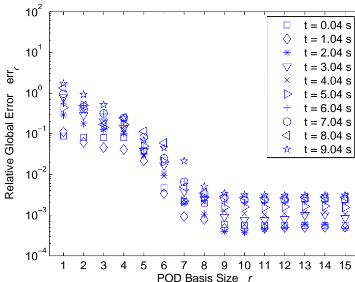
Figure 3: Semilog plot of relative global error versus POD basis size at various points in time for the simulation of the standard POD model of the fluctuation Burgers' equation
