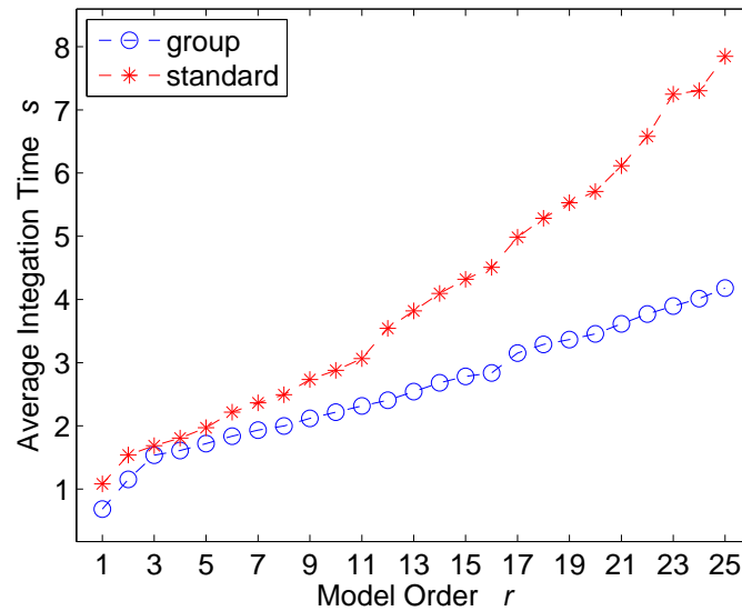
Figure 6: Total integration time (averaged over 100 trials) of standard and group POD models of Burgers equation versus model order
