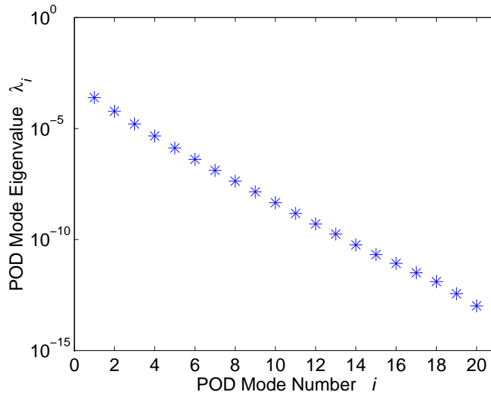
Figure 5: POD eigenvalues 1 to 20 computed from a 33 \times 33 node 1025 snapshot snapshot set of the unforced GFE simulation of Burgers' equation (10)
