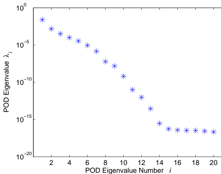
Figure 1: POD eigenvalues 1 to 20 computed from a 1025 snapshot 65 \times 65 node snapshot set of the benchmark solution (36)
