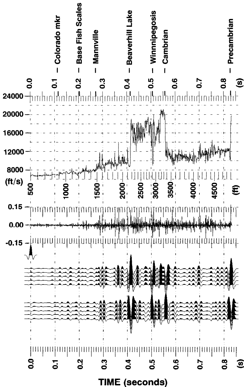
FIG. 9. Velocity log (top); reflectivity log; a zero-phase, 20-ms, 39-Hz Ricker wavelet; and normal- and reverse-polarity (bottom) synthetic seismograms for the 6-5-51-2OW3M well generated using this Ricker wavelet. This well did not encounter any residual Leofnard rock salt.
