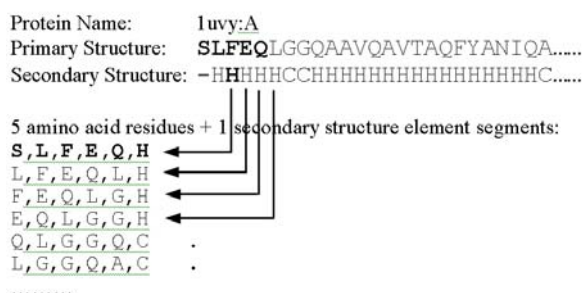
Note: The first and second positions at the beginning of the sequence are represented by 3 residues + 1, and 4 residues + 1 segments, respectively. They form separate training datasets.
