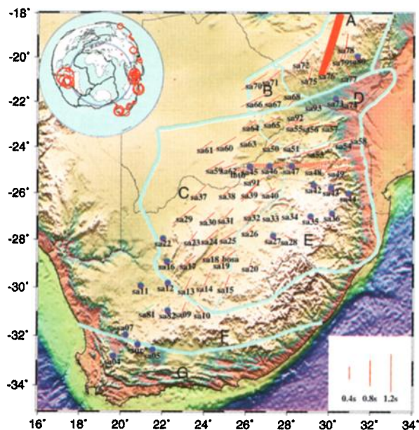
Figure 1. Shear-wave splitting measurements. Orientation, length of bars give fast polarization direction, splitting delay time, respectively, for Type I (red, high-quality) and III (blue, low-quality) stations. Purple dots denote undetectable splitting (Type II). Also shown, tectonic domains. Area A: Zimbabwe craton near Great Dyke. Area B: southwestern corner of Zimbabwe craton. Area C: western half of Kaapvaal craton. Area D: Limpopo belt. Area E: southeastern Kaapvaal craton. Area F: Namaqua–Natal mobile belt. Area G: Cape fold belt. Ages: A–D, Late-Archean; E, Early-Archean; F, G younger than 2.0 Ga (see text). Solid red line (Area A) denotes Great Dyke. Dashed red line denotes Murchison Lineament. Small inset, top-left: Events used in study. Circle size proportional to number of records used from event.
